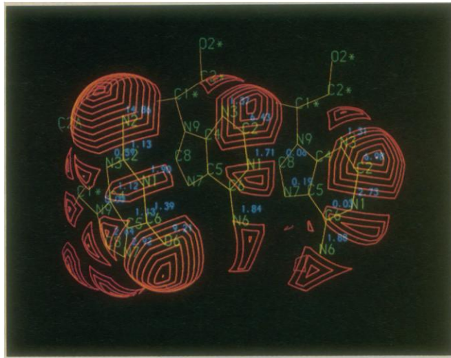
Fig. 3 (left). Trajectory of probe rolling over a molecular surface. The trajectory arcs (red) connect positions where the probe is simultaneously tangent to three atoms. In a corresponding manner, saddle rectangles connect concave triangles. These reentrant surfaces (green) then define the boundaries of the convex surfaces (magenta). Fig. 4 (right). Yeast phenylalanyl transfer RNA anticodon (GAA). The contact surface of the three anticodon bases is shown. The contact areas in square angstroms are displayed next to the atom labels.
